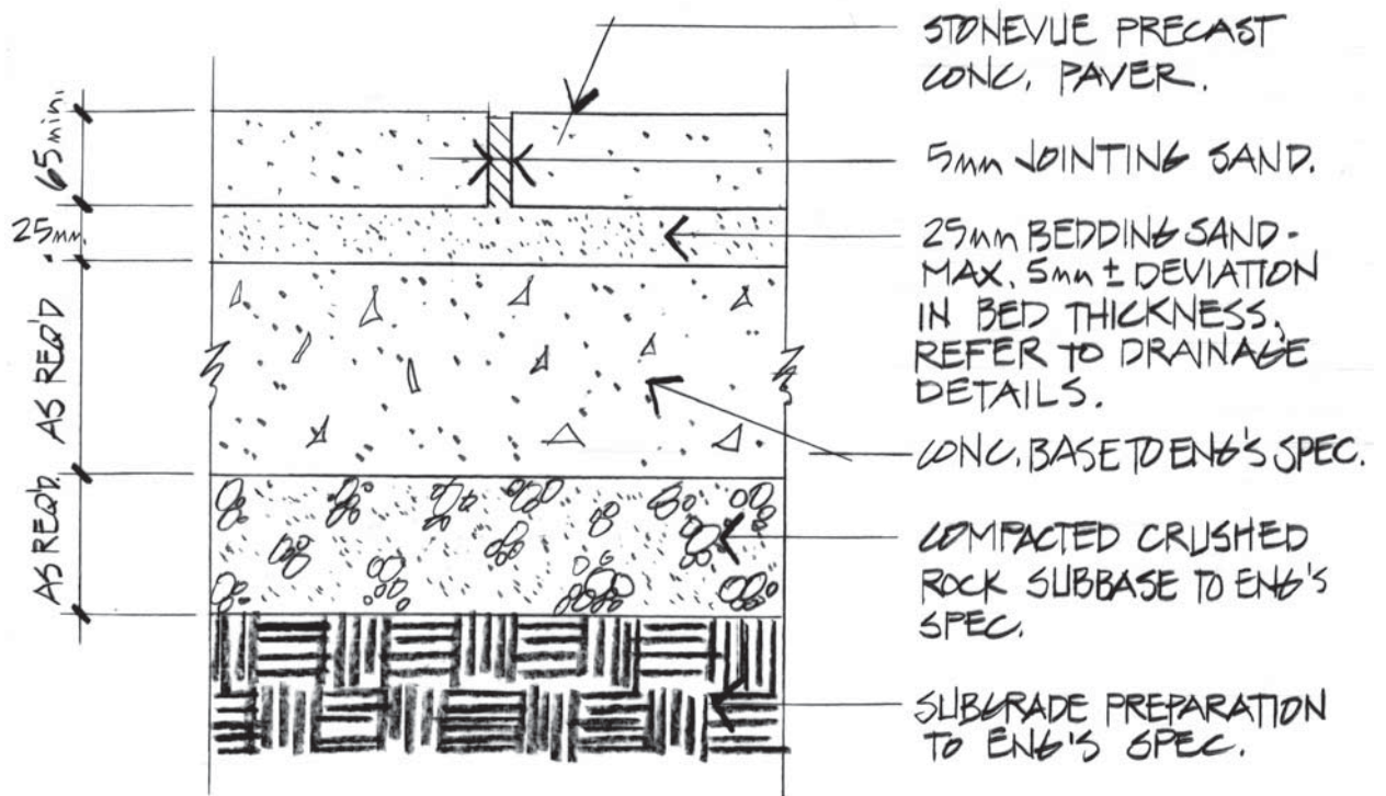
SECTION - VEHICULAR STONEVUE CONCRETE BASE PAVING SYSTEM 1/5
