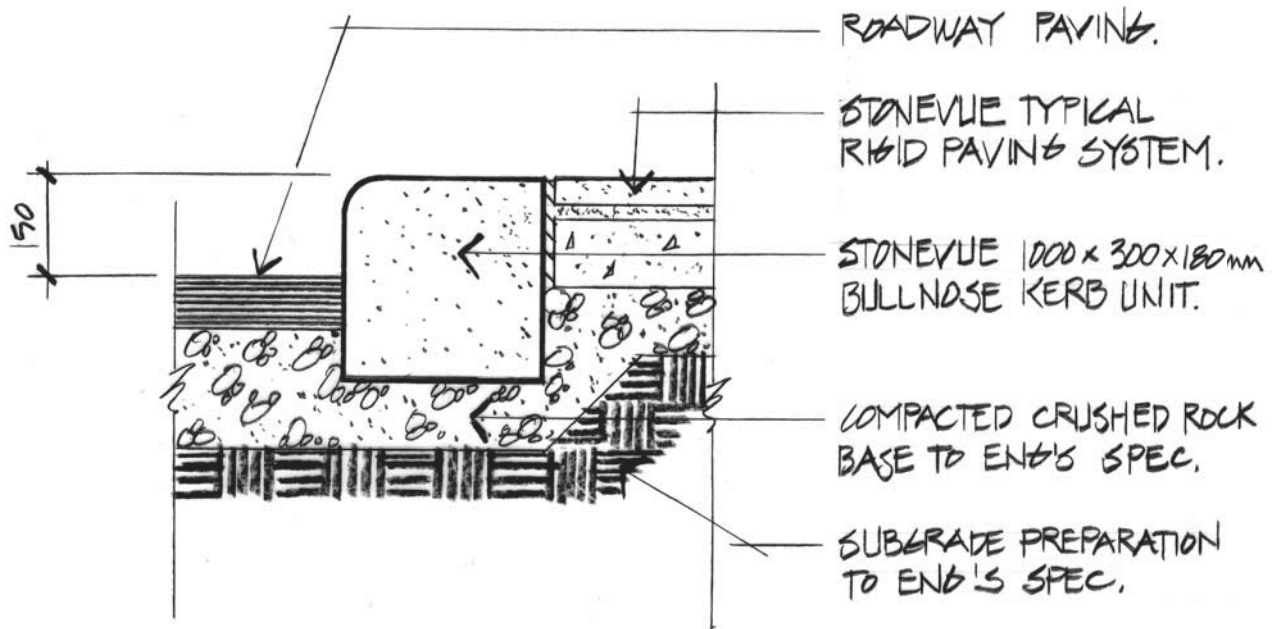
SECTION STONEVUE BULLNOSE KERB
